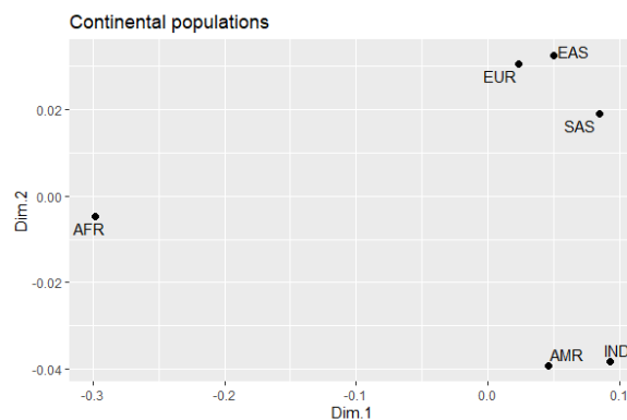
Figure 1. Multidimensional scaling plot illustrating the grouping of ethnic populations according to the genetic profile of the 15 variants in the BRCA1 and BRCA2 genes.
